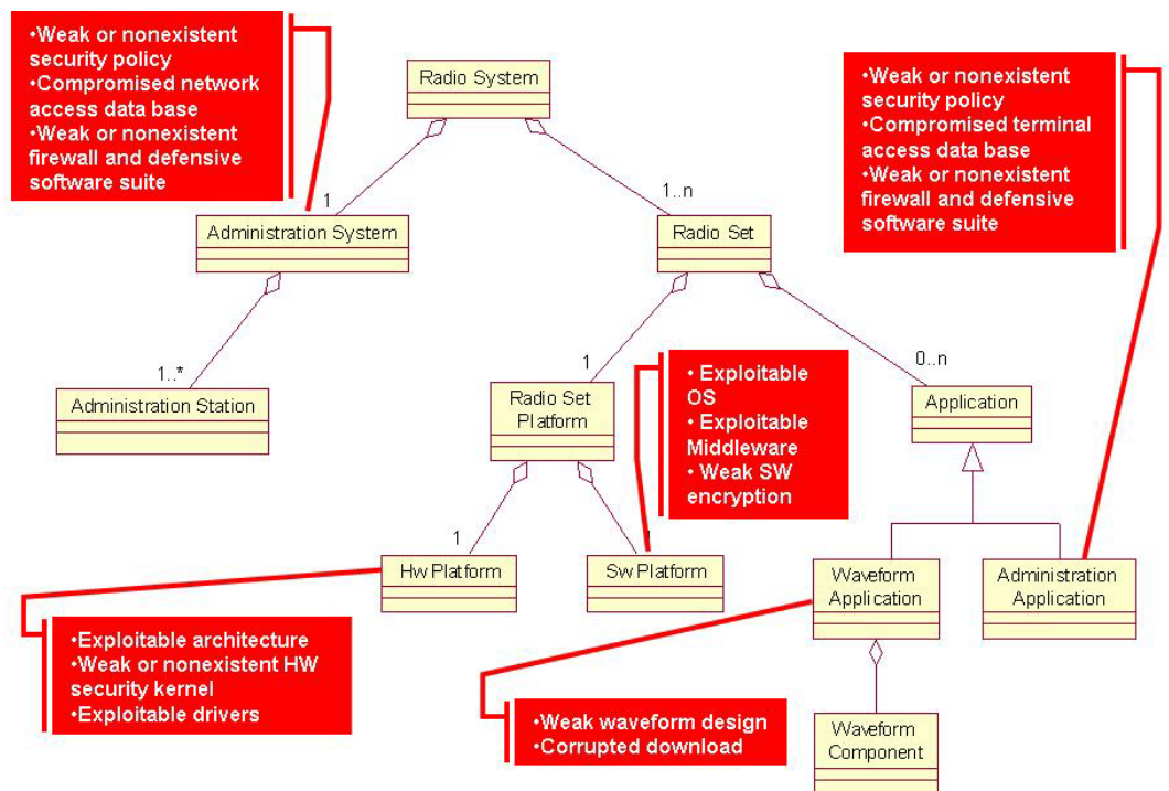
Figure 1. Potential vulnerabilities of SDR System, from [3].
